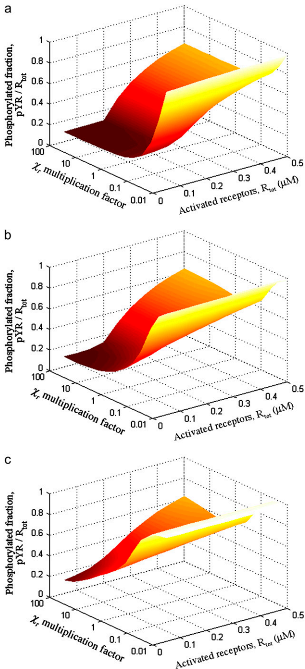
FIGURE 4 Intracomplex binding is important for high-avidity binding of Shp2. The fraction of activated receptors phosphorylated on the Shp2 substrate site, Y_1 ( p_{YR}/R_{tot} ), was calculated as a function of the abundance of activated receptors ( R_{tot} ) and the intracomplex association rate constants (varied by multiplying the base-case values of \chi_r , listed in Table 2, by a common factor). The value of k_{off,CSH2} = k_{off,NSH2} = k_{off} was varied according to (a) k_{off} = 0.1 \text{ s}^{-1} ; (b) k_{off} = 1.0 \text{ s}^{-1} ; (c) k_{off} = 5.0 \text{ s}^{-1} . In all cases, S_{tot} = 0.10 \text{ } \mu\text{M} , and other parameter values are as listed in Table 1.
